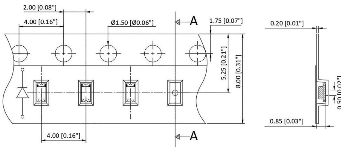
7：包装规格图 (drawing 7: packing specification)
